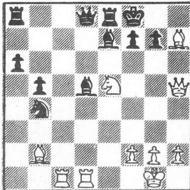
306 After 20...Bxd5
